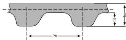
梯形齿 T TOOTH
