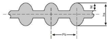
圆弧双面齿 DOUBLE SIDED ARC TOOTH
