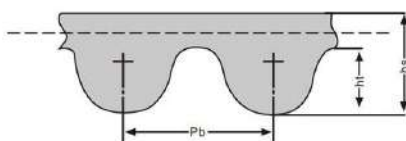
HTD 圆弧齿 HTD ARC TOOTH
