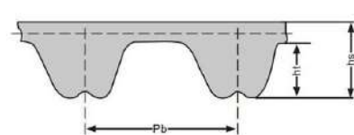
EPP/HPPD 圆弧齿 RPP/HPPD ARC TOOTH
