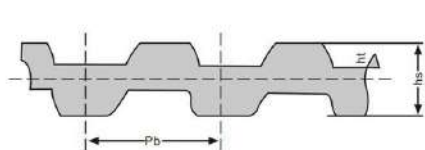
梯形双面齿 DOUBLE T TOOTH
