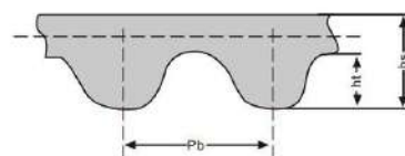
STPD/STS 圆弧齿 STPD/STS ARC TOOTH
